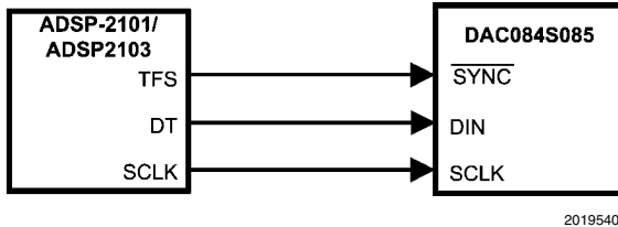
FIGURE 10. ADSP-2101/2103 Interface
